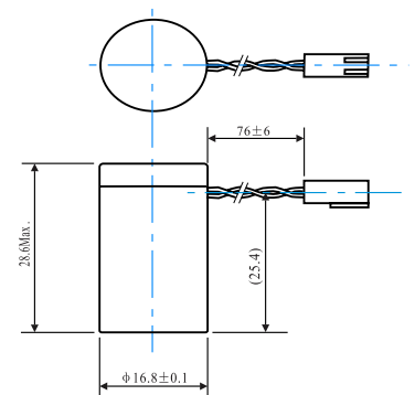
Case Type
