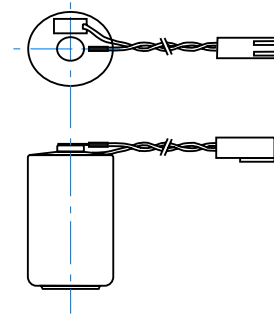
Connector Type 2
